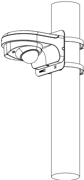
Pole Mount(Vertical)
