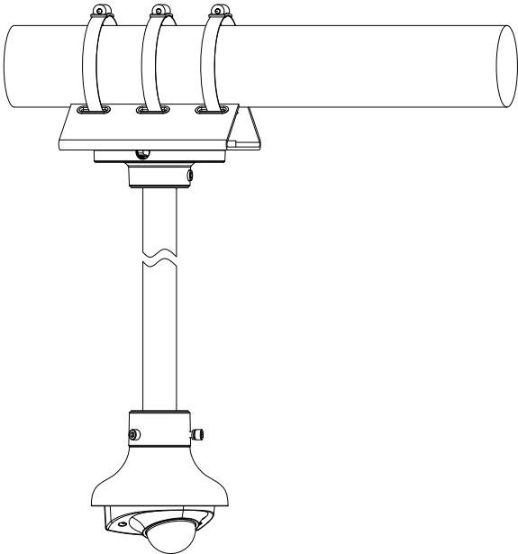
Pole Mount(Horizontal)
