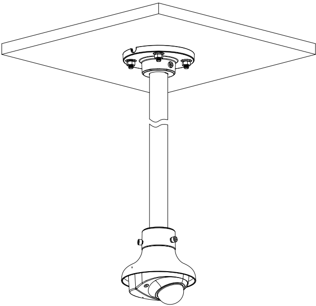
Pole Mount(Vertical)
